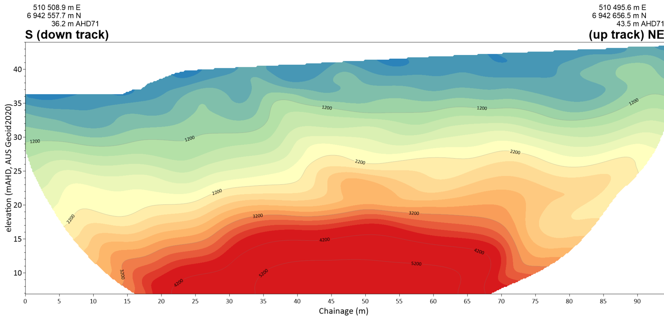
Seismic Line SR AU-GP 130
